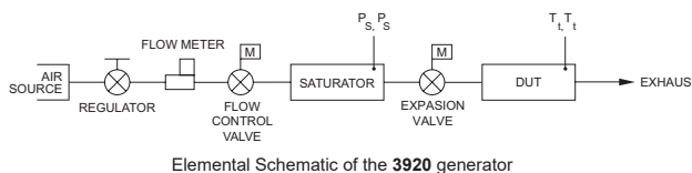
Elemental Schematic of the 3920 generator
